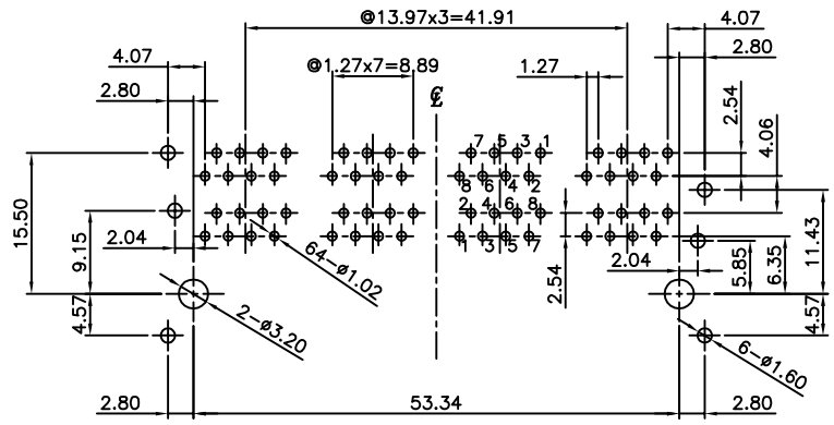
PC Board Layout Component Side Shown PC Board Thickness=2.0mm
