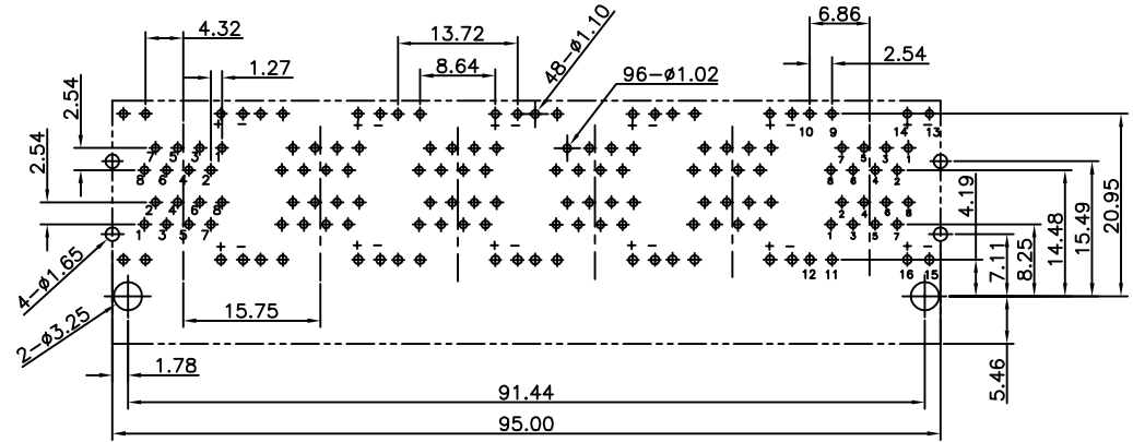
PC Board Layout Component Side Shown PC Board Thickness=1.6mm Tolerance±0.05
